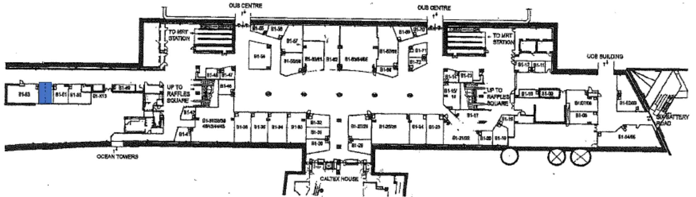
RAFFLES XCHANGE FLOOR PLAN
