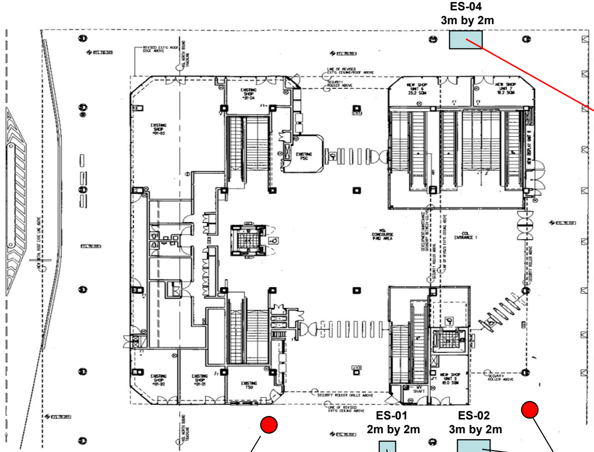
CONCOURSE LEVEL PLAN - BISHAN MRT STATION (FLOOR PLAN AND AREA - SUBJECT TO CHANGES)
