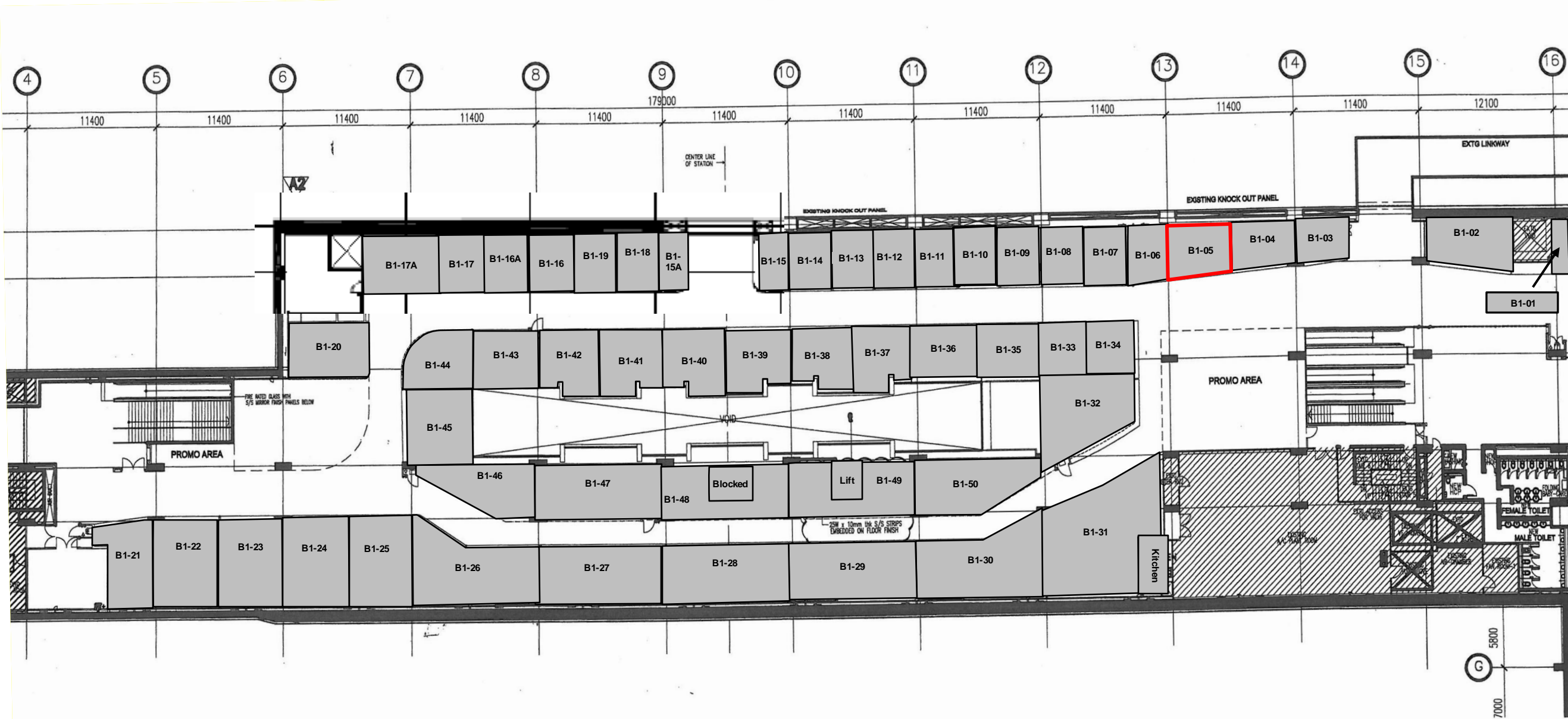
① BASEMENT 1 - CONCOURSE LEVEL SHOP UNIT LIST WITH FLOOR AREA SCALE 1:300m
